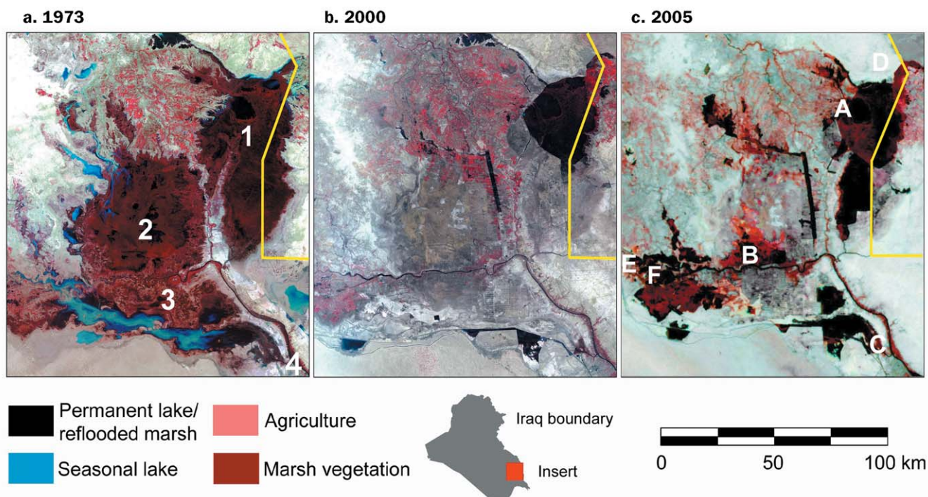
Figure 1. (a) A composite view of the Mesopotamian marshlands from a mosaic of four Landsat 1 images and two false-color, near-infrared images, 1973–1976. Dense marsh vegetation (mainly Phragmites australis ) appears in dark red, seasonal lakes in blue, agriculture in pink, and permanent lakes in black. The red elongated patches along riverbanks are date palms. The three main marsh areas are Al-Hawizeh, Central, and Al-Hammar, labeled 1, 2, and 3, respectively. The city of Basrah is located at number 4. Modified from Richardson and colleagues (2005). (b) A Landsat 7 Enhanced Thematic Mapper mosaic taken in 2000. Most of the drained marshes appear as grayish-brown patches, indicating dead marsh vegetation or low desert shrubs and dry ground. The white and gray patches indicate bare areas with no vegetation and, in some areas, salt evaporites or shells covering the bottoms of former lakes. By 2000, 85% of the 8926 square kilometers ( \text{km}^2 ) of permanent marsh in 1973 marshlands had been destroyed. Only 3% of the Central marsh and 14.5% of the Al-Hammar remained. A canal known as the Glory River (shown as a straight line across the top and down the east side of the Central marsh), constructed in 1993, completely dried up the Central marsh by stopping water inflow from the Tigris River. The largest expanse (approximately 1025 \text{ km}^2 ) of remaining natural marsh, the Al-Hawizeh, near the Iranian border, is shown in dark red. Modified from Richardson and colleagues (2005). (c) False-color image of the remaining Mesopotamian marshlands, taken 2 September 2005, shows in black the areas newly reflooded since the war. Reflooded areas adjacent to Al-Hawizeh, the western area of Al-Hammar, and waterways in the northern and southern parts of the Central marsh are also visible in black. Al-Hawizeh (called Hawr Al-Azim in Iran) is the best remaining natural marsh in the region. It straddles the Iraq–Iran border (yellow line). During a field survey in February 2004, we discovered an Iranian dike under construction that is now nearly completed and will traverse directly through the Al-Hawizeh marsh, along the Iraq–Iran border, and, as a result, will significantly reduce the water input from the Karkheh and Karun rivers to the marsh. The ecological affects of this massive water diversion are unknown, but it will significantly affect the last remaining natural marsh system in Iraq. Sampling sites: A, Al-Hawizeh; B, Central; C, Al-Hammar; D, Al-Sanaf; E, Abu Zarag; F, Suq Al-Shuyukh. MODIS satellite image courtesy of the United Nations Environment Programme, Iraq Marshlands Observation System.
